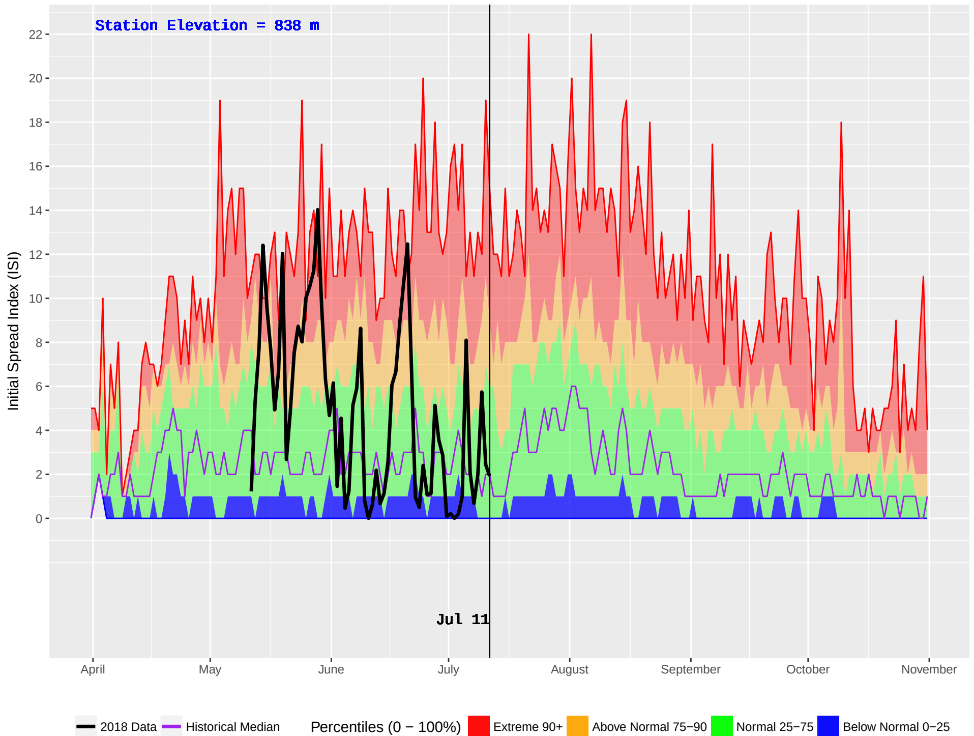
HOWARD (343) : Historical (1970–2016) and Current (2018) Daily Initial Spread Index (ISI)
